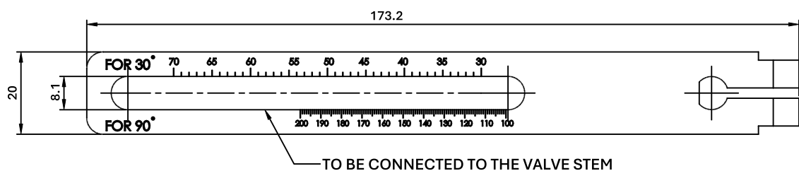
LINEAR SCALE TYPE 2 (100 - 200 MM STROKE) DETAIL VIEW
