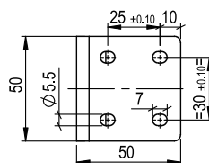
BRACKET FOR PINION HEIGHT 20MM
